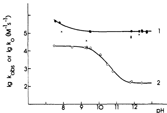
Figure 4. Second-order rate constant for the faster ( k_{\text{obs}} , curve 1) and the slower ( k_0 , curve 2) phase of sulfite oxidation at 20 °C, as a function of pH. The X's are k_{\text{obs}} values obtained with ionic strengths far below 0.1 M (see Table I).
