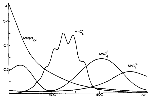
Figure 1. UV-vis. spectra of manganese species in the oxidation states VII–IV: 2 \times 10^{-4} M solutions; 1-cm cells; t = 20^\circ\text{C} .
